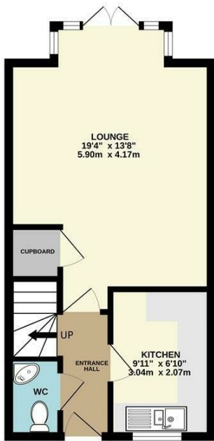
GROUND FLOOR 365 sq.ft. (33.9 sq.m.) approx.
